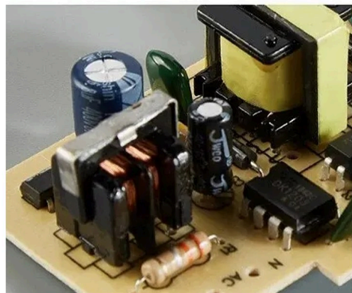
EMI Filter
